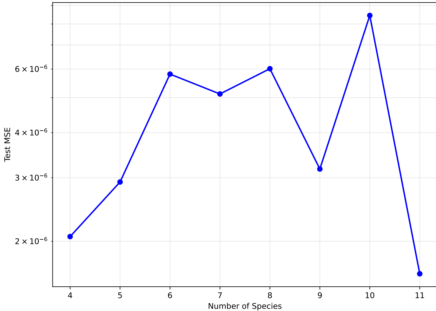
30, 30 — Test MSE vs number of species (zoomed: 4 to 11 species)
